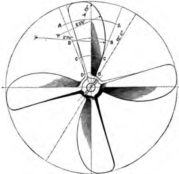
Fig. 189.—Screw-Propeller.
